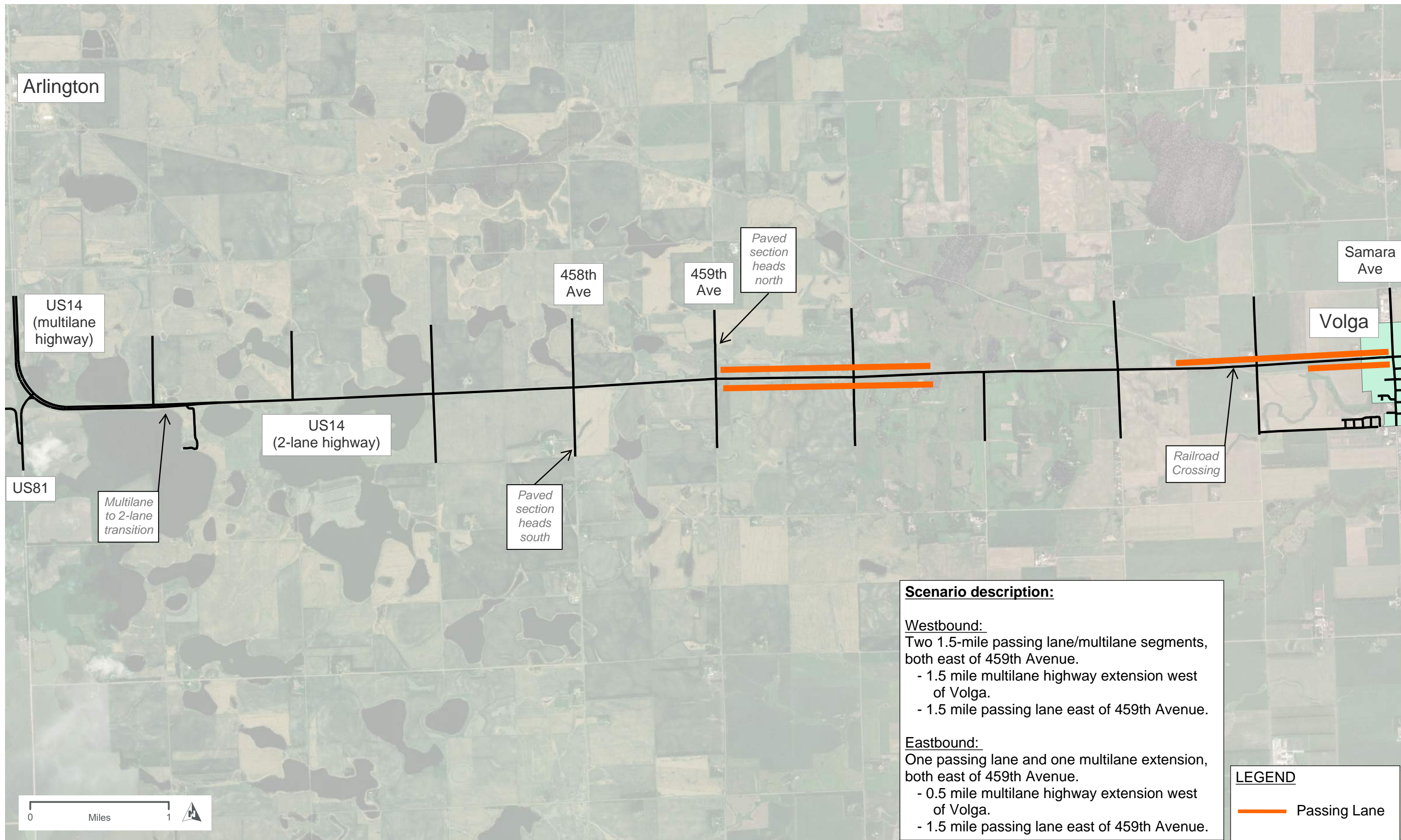
Passing Lane Scenario B US14-US14 BYPASS CORRIDOR STUDY
